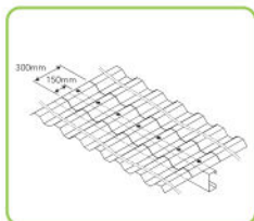
Sidelap - Vermax® Lite Roofing Sheets Lap Over Metal Roof
